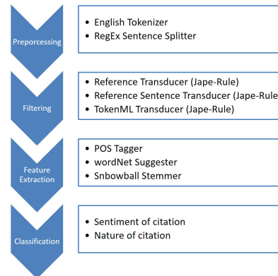
Figure 1: Complete workflow for SentiCite.
