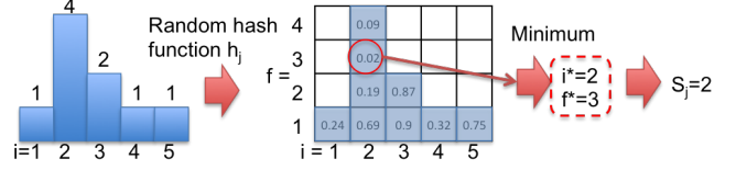
Figure 2: An example of sketch creation
